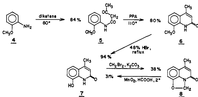
Figure 1. Preparation and reactions of 6-methyl-2H,4H-oxazolo[5,4,3-ij]quinolin-4-one (8); PPA = polyphosphoric acid.
