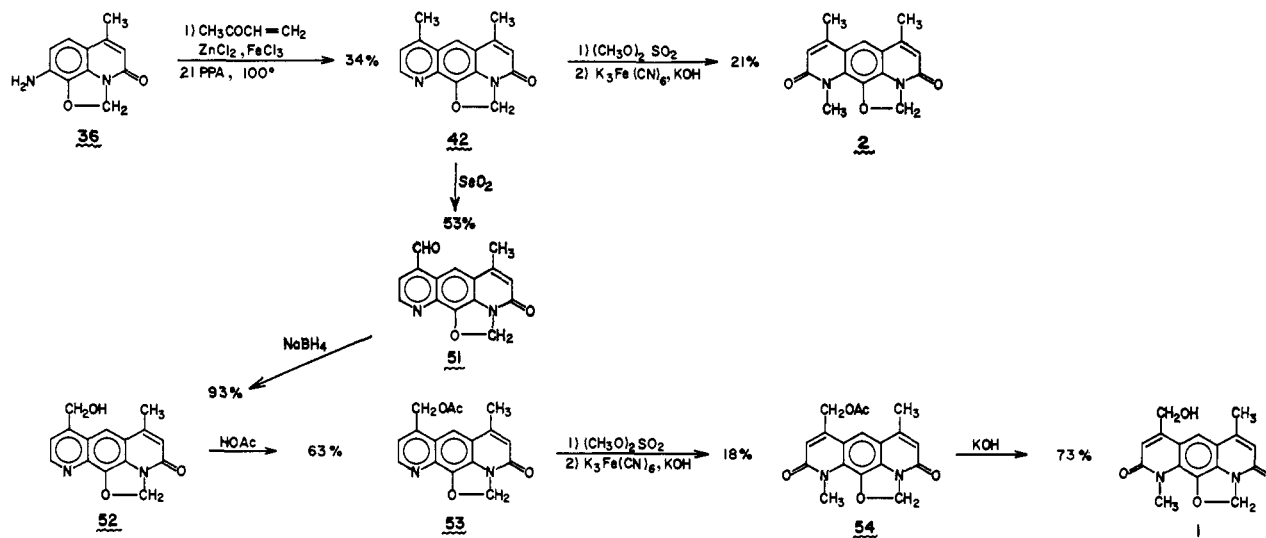
Figure 5. Syntheses of deoxynybomycin (2) and nybomycin (1).
