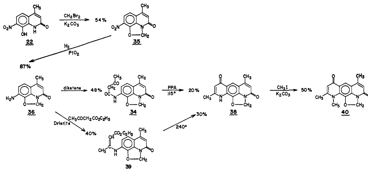
Figure 4. Preparation of isodeoxybomycin (40).
